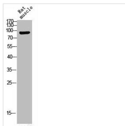
Western Blot analysis of RAT-MUSCLE cells using Phospho-Trk B (Y516) Polyclonal Antibody
