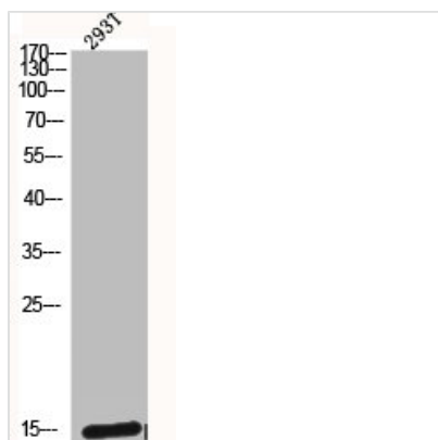
Western Blot analysis of 293T cells using Bcl-2 Polyclonal Antibody
