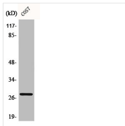
Western Blot analysis of COS7 cells using Bcl-2 Polyclonal Antibody
