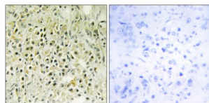
Immunohistochemistry analysis of paraffin-embedded human prostate carcinoma tissue, using LEG8 antibody.
