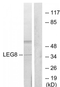
Western blot analysis of extracts from 3T3 cells, using LEG8 antibody.
