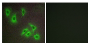
Immunofluorescence analysis of HepG2 cells, using BCLW antibody.
