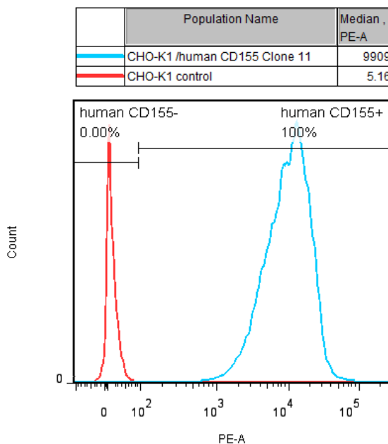
Figure 1. FACS analysis of CD155 expression in CHO-K1 cells.
