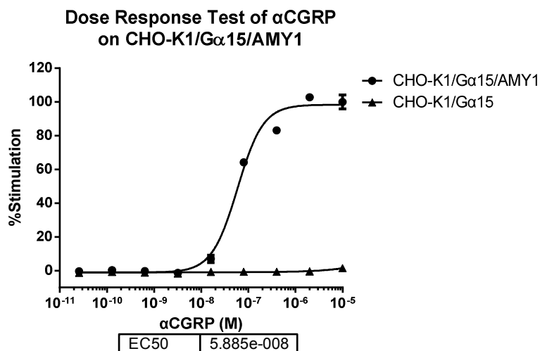
Figure 1. \alpha -CGRP-induced concentration-dependent stimulation of intracellular calcium mobilization in CHO-K1/ G_{\alpha 15} /AMY1 and CHO-K1/ G_{\alpha 15} cells. The cells were loaded with Calcium-4 prior to stimulation with an AMY1 receptor agonist, \alpha -CGRP. The intracellular calcium change was measured by FlexStation. The stimulation% were plotted against the log of the cumulative doses (5-fold dilution) of \alpha -CGRP (Mean \pm SD, n = 4). The EC 50 of \alpha -CGRP on AMY1 expressing in CHO-K1/ G_{\alpha 15} cells was 58.8 nM.
