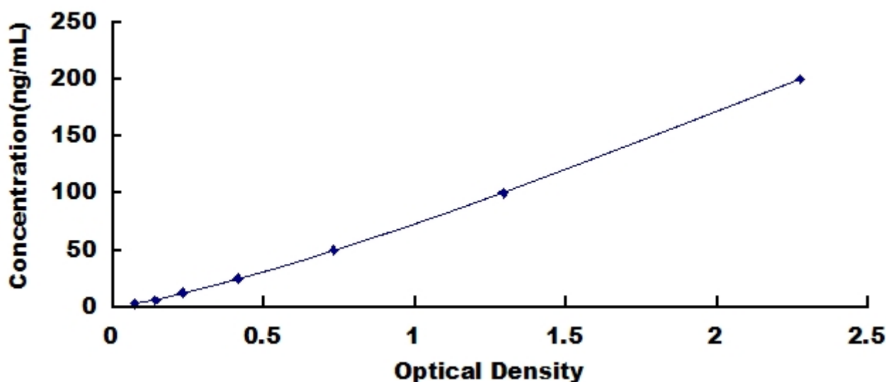
Typical Standard Curve for FBLN1, Human ELISA.
