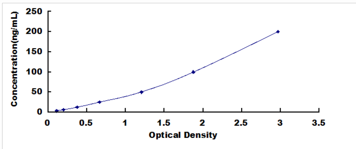
Typical Standard Curve for CLU, Canine ELISA.
