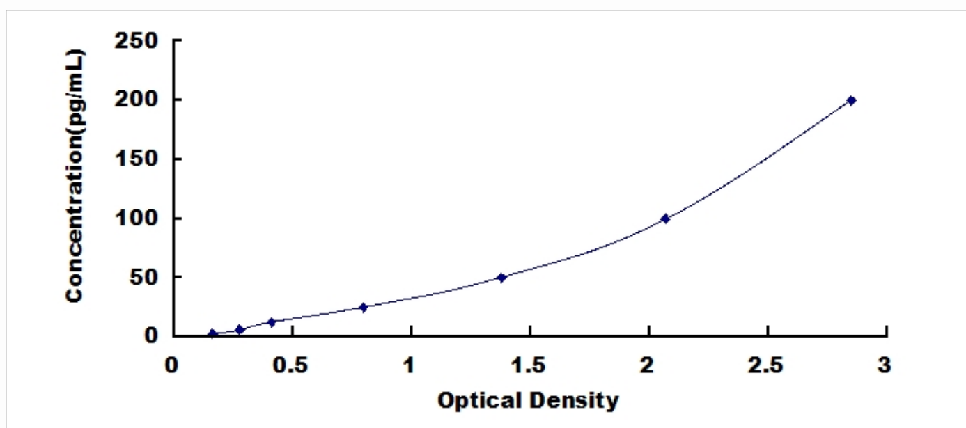
Typical Standard Curve for IFN \beta , Gallus ELISA.
