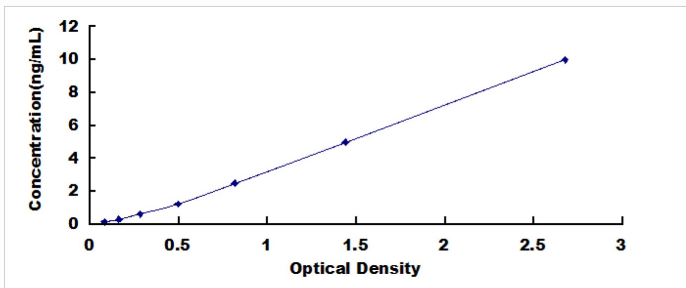
Typical Standard Curve for uPA, Porcine ELISA.
