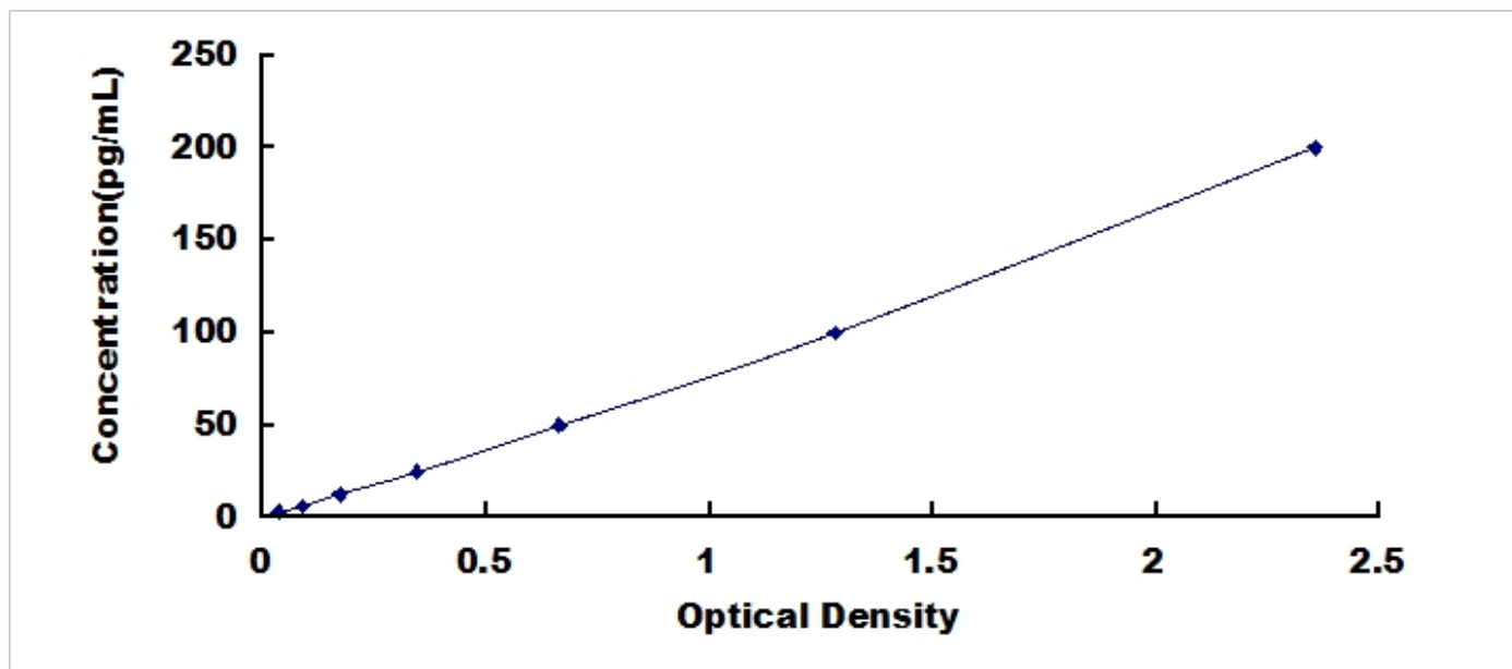
Typical Standard Curve for NT3, Rat ELISA.
