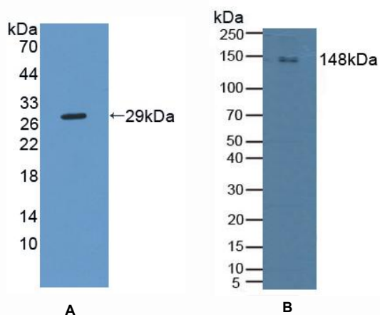
Figure 1. Western Blot
