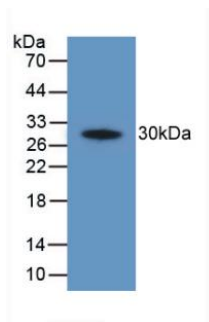
Figure. Western Blot; Sample: Recombinant PTGS2, Human.
