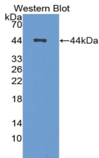
Figure. Western Blot; Sample: Recombinant BDNF, Cavia.
