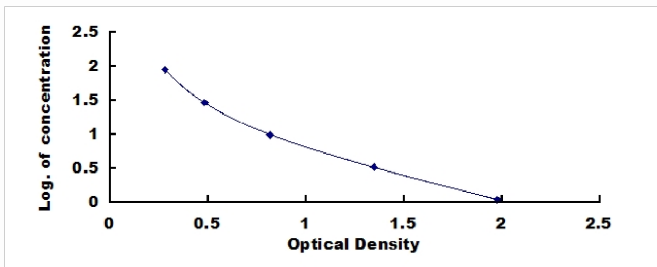
Typical Standard Curve for FSH, Human ELISA.
