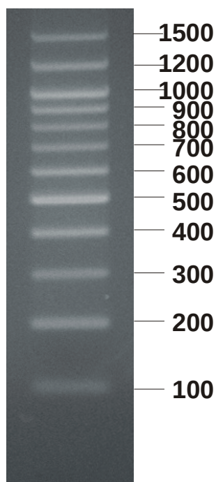
2% Agarose Gel
