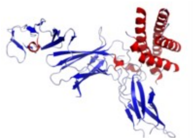
Crystal structure of human IL-12
