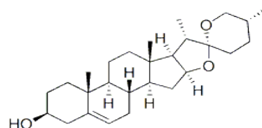
Chemical Structure
